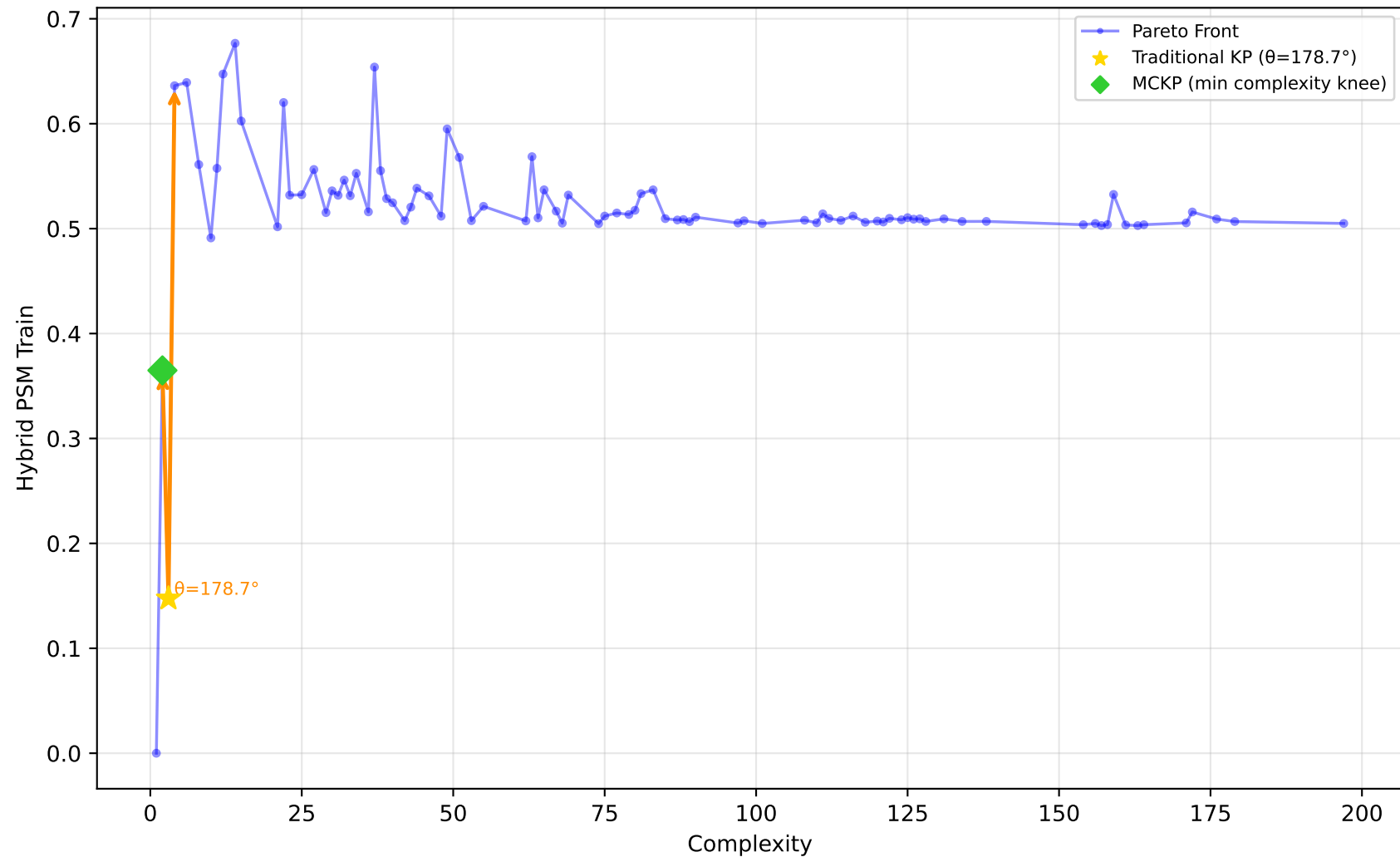
561_cpu - Run 3 - SVP - Hybrid PSM Train \lambda_1=1.00, \lambda_2=0.00, \lambda_3=0.40 | Difficulty: 1.00 | Method: hmr
