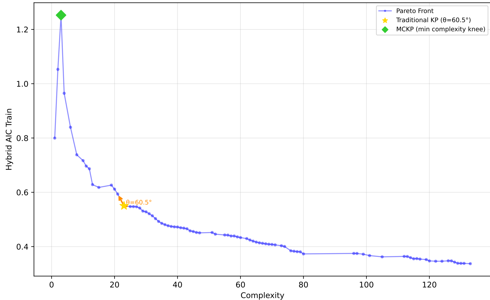
561_cpu - Run 4 - MVP - Hybrid AIC Train \lambda_1=0.50, \lambda_2=0.20, \lambda_3=0.00 | Difficulty: 1.00 | Method: hmr
