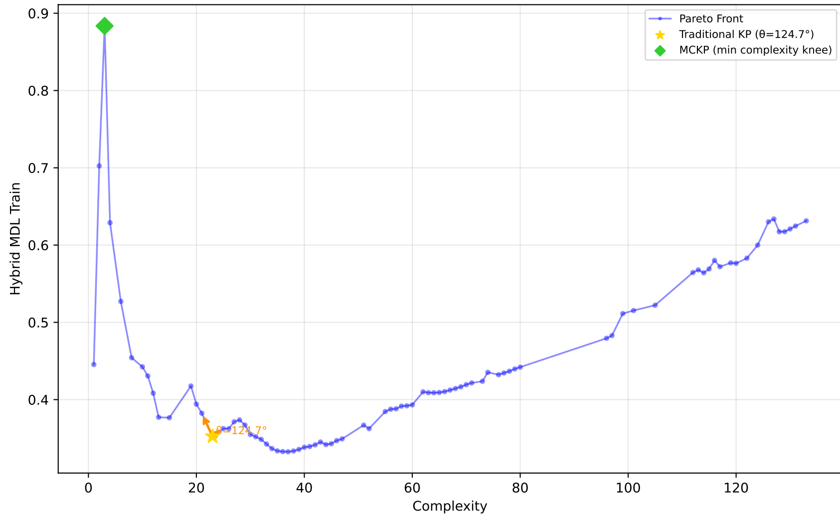
561_cpu - Run 4 - MVP - Hybrid MDL Train \lambda_1=0.50, \lambda_2=0.20, \lambda_3=0.00 | Difficulty: 1.00 | Method: hmr
