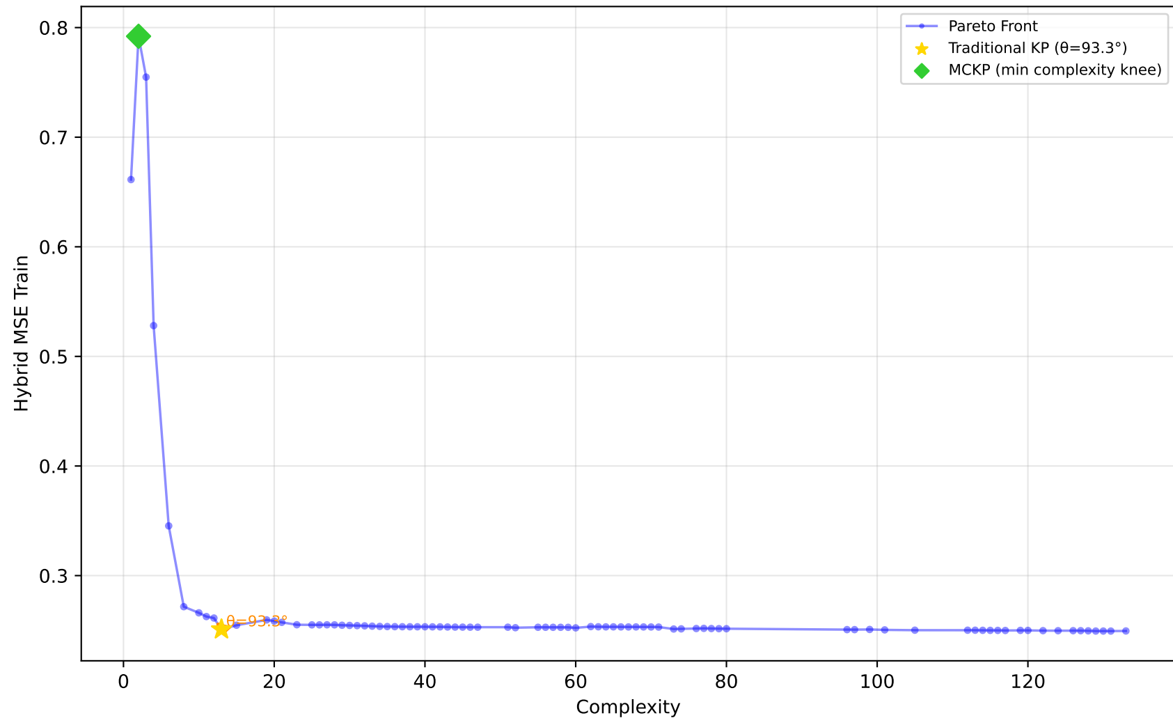
561_cpu - Run 4 - MVP - Hybrid MSE Train \lambda_1=0.50, \lambda_2=0.20, \lambda_3=0.00 | Difficulty: 1.00 | Method: hmr
