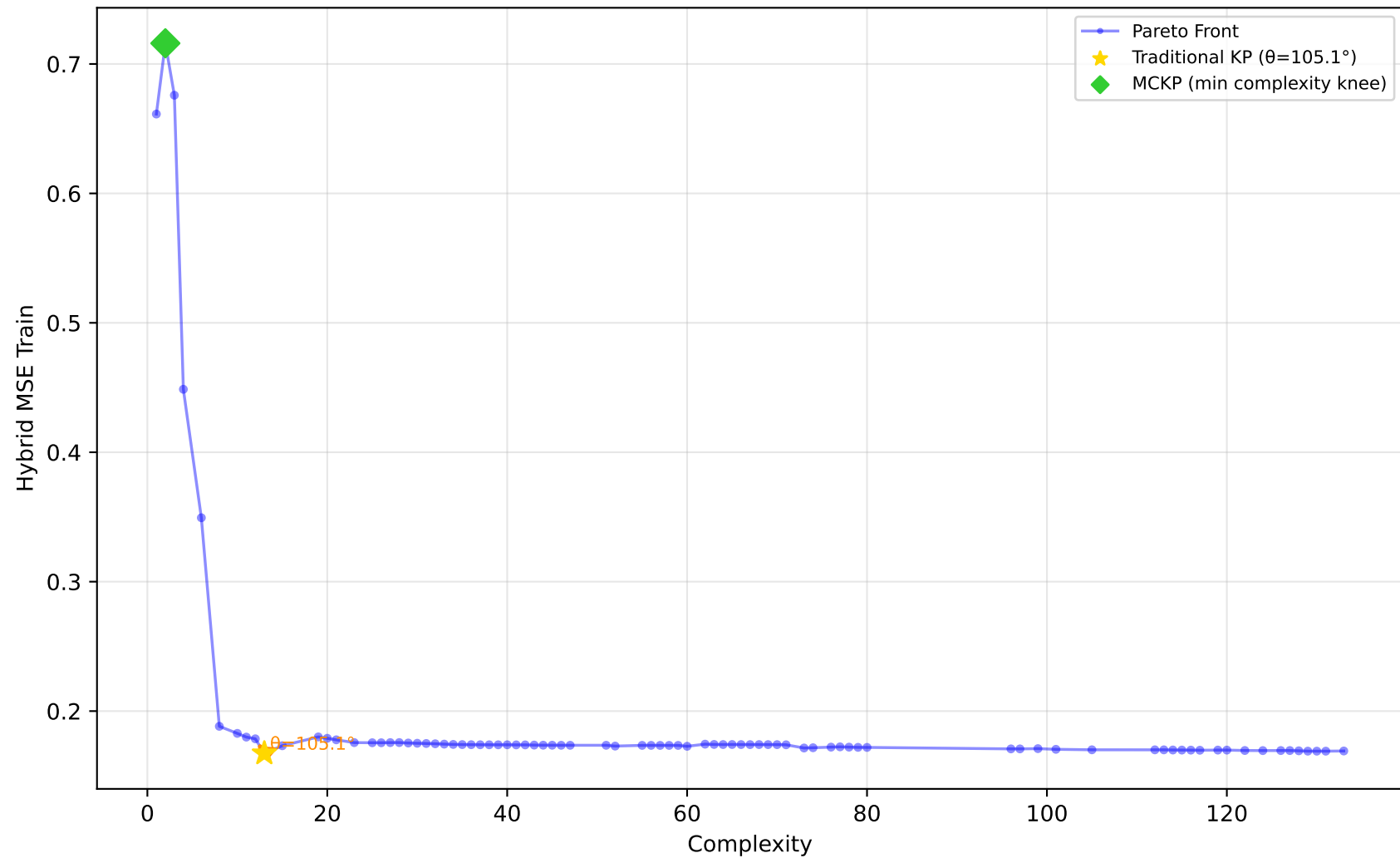
561_cpu - Run 4 - MVP - Hybrid MSE Train \lambda_1=0.70, \lambda_2=0.00, \lambda_3=0.10 | Difficulty: 1.00 | Method: hmr
