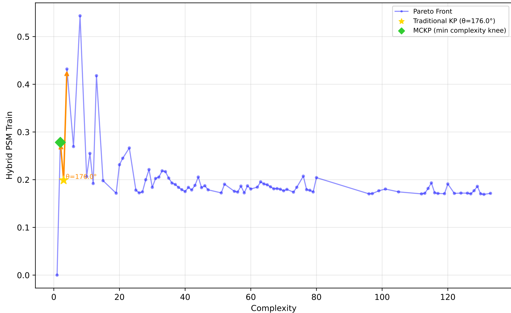
561_cpu - Run 4 - MVP - Hybrid PSM Train \lambda_1=0.70, \lambda_2=0.00, \lambda_3=0.10 | Difficulty: 1.00 | Method: hmr
