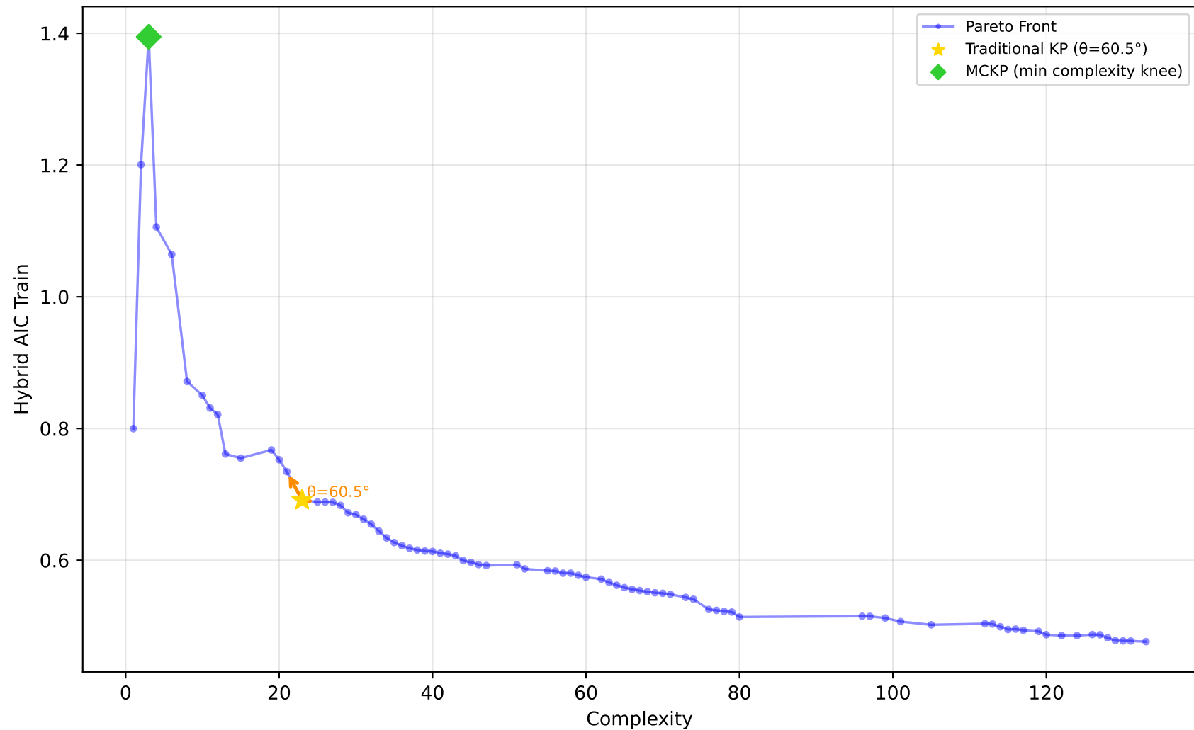
561_cpu - Run 4 - SVP - Hybrid AIC Train \lambda_1=0.90, \lambda_2=0.00, \lambda_3=0.30 | Difficulty: 1.00 | Method: hmr
