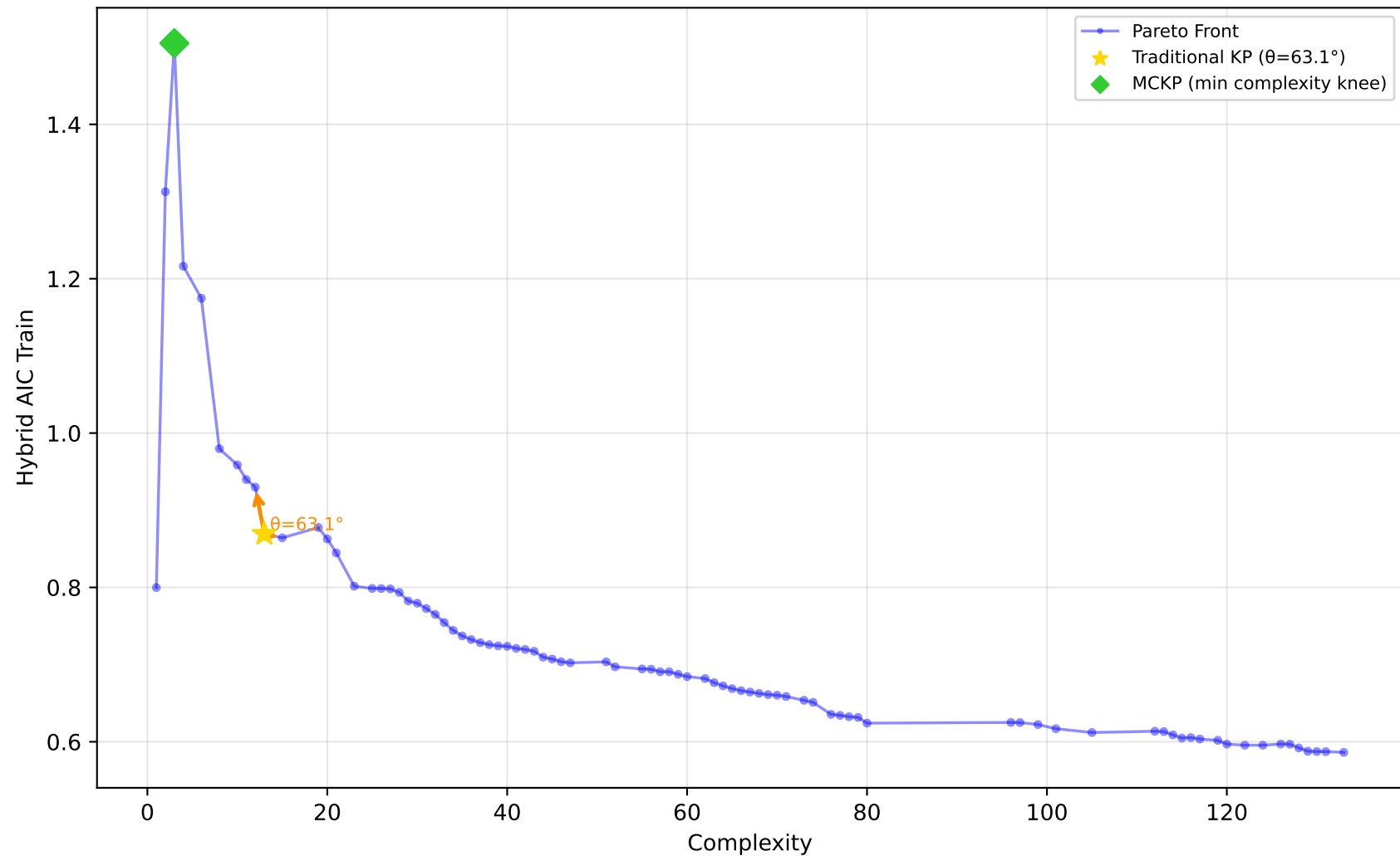
561_cpu - Run 4 - SVP - Hybrid AIC Train \lambda_1=1.00, \lambda_2=0.00, \lambda_3=0.40 | Difficulty: 1.00 | Method: hmr
