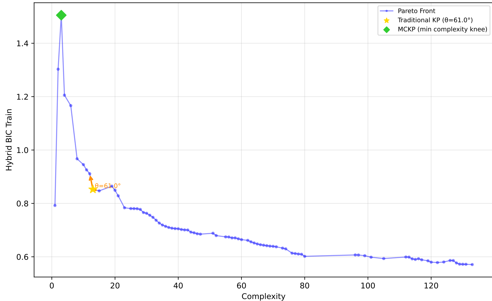
561_cpu - Run 4 - SVP - Hybrid BIC Train \lambda_1=1.00 , \lambda_2=0.00 , \lambda_3=0.40 | Difficulty: 1.00 | Method: hmr
