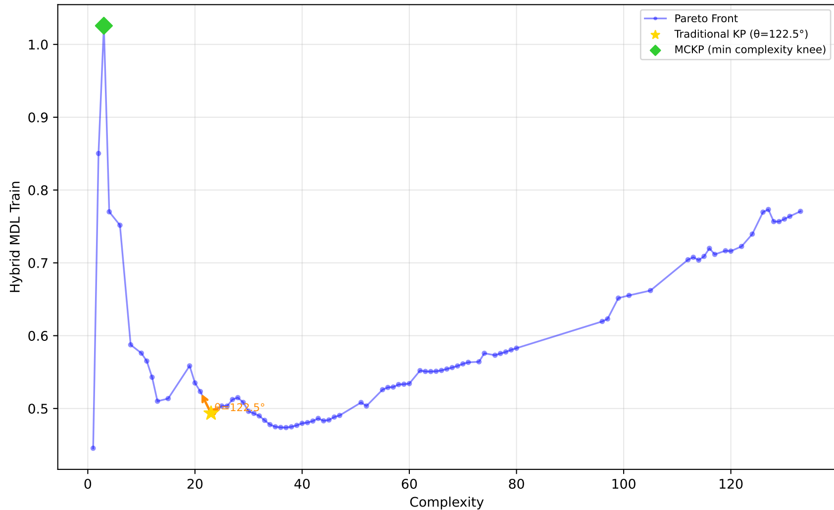
561_cpu - Run 4 - SVP - Hybrid MDL Train \lambda_1=0.90, \lambda_2=0.00, \lambda_3=0.30 | Difficulty: 1.00 | Method: hmr
