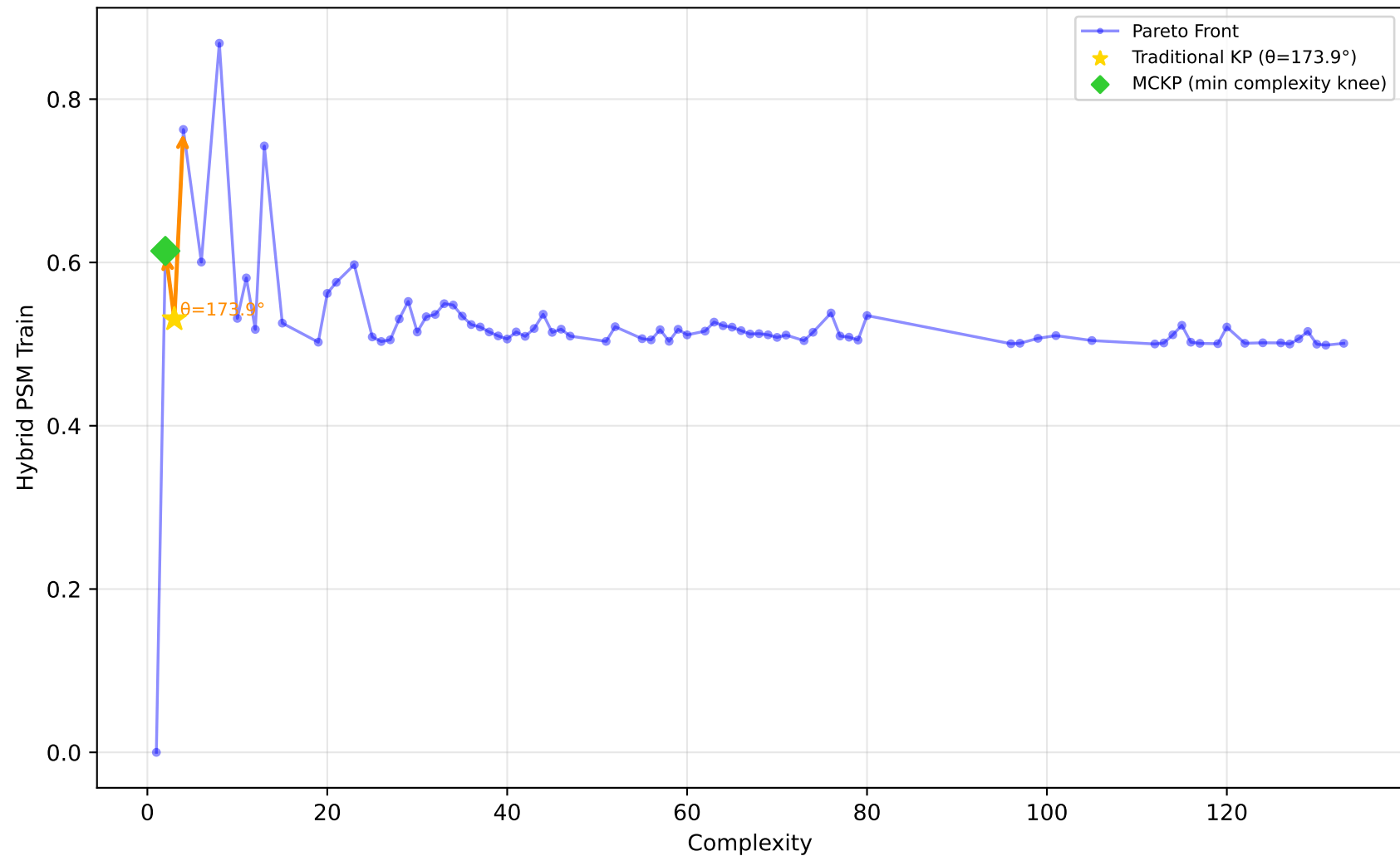
561_cpu - Run 4 - SVP - Hybrid PSM Train \lambda_1=1.00, \lambda_2=0.00, \lambda_3=0.40 | Difficulty: 1.00 | Method: hmr
