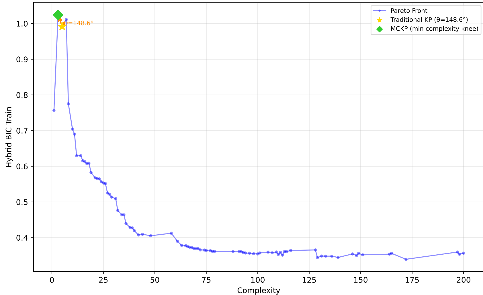
561_cpu - Run 5 - MVP - Hybrid BIC Train \lambda_1=0.50, \lambda_2=0.20, \lambda_3=0.00 | Difficulty: 1.00 | Method: hmr
