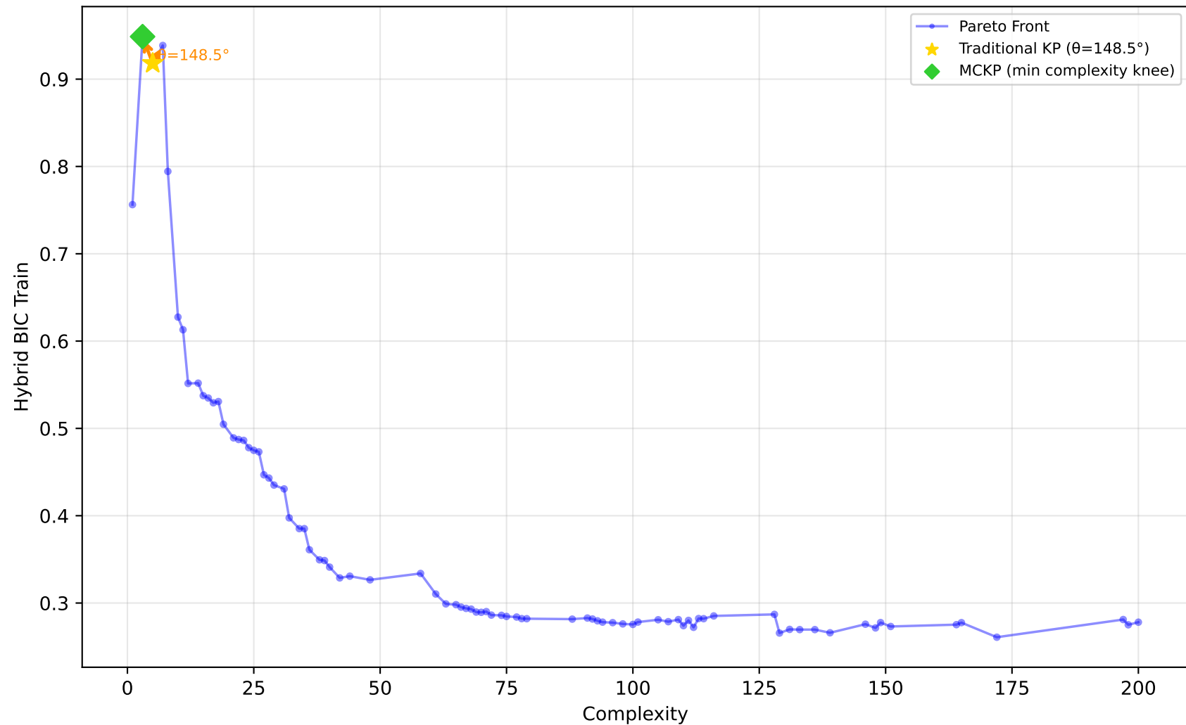
561_cpu - Run 5 - MVP - Hybrid BIC Train \lambda_1=0.70, \lambda_2=0.00, \lambda_3=0.10 | Difficulty: 1.00 | Method: hmr
