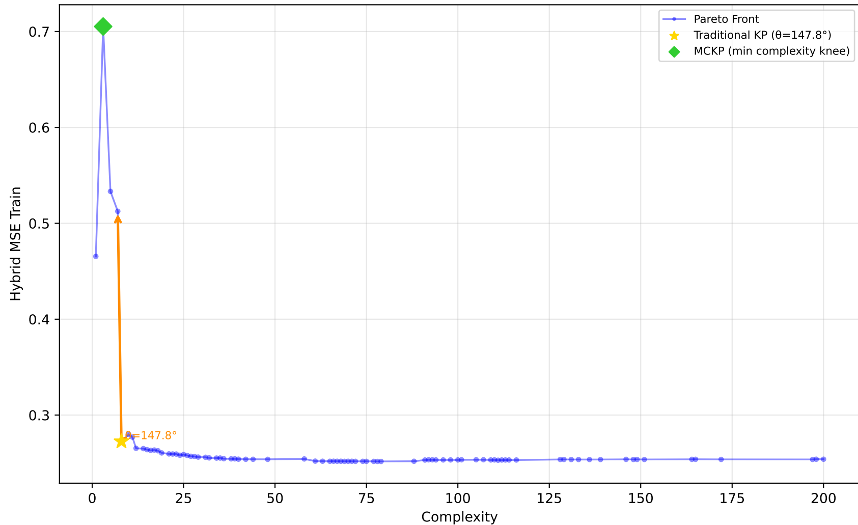
561_cpu - Run 5 - MVP - Hybrid MSE Train \lambda_1=0.50, \lambda_2=0.20, \lambda_3=0.00 | Difficulty: 1.00 | Method: hmr
