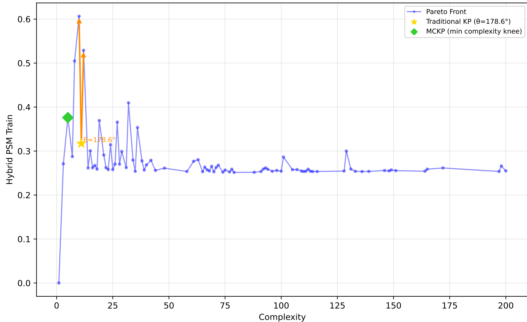
561_cpu - Run 5 - MVP - Hybrid PSM Train \lambda_1=0.50, \lambda_2=0.20, \lambda_3=0.00 | Difficulty: 1.00 | Method: hmr
