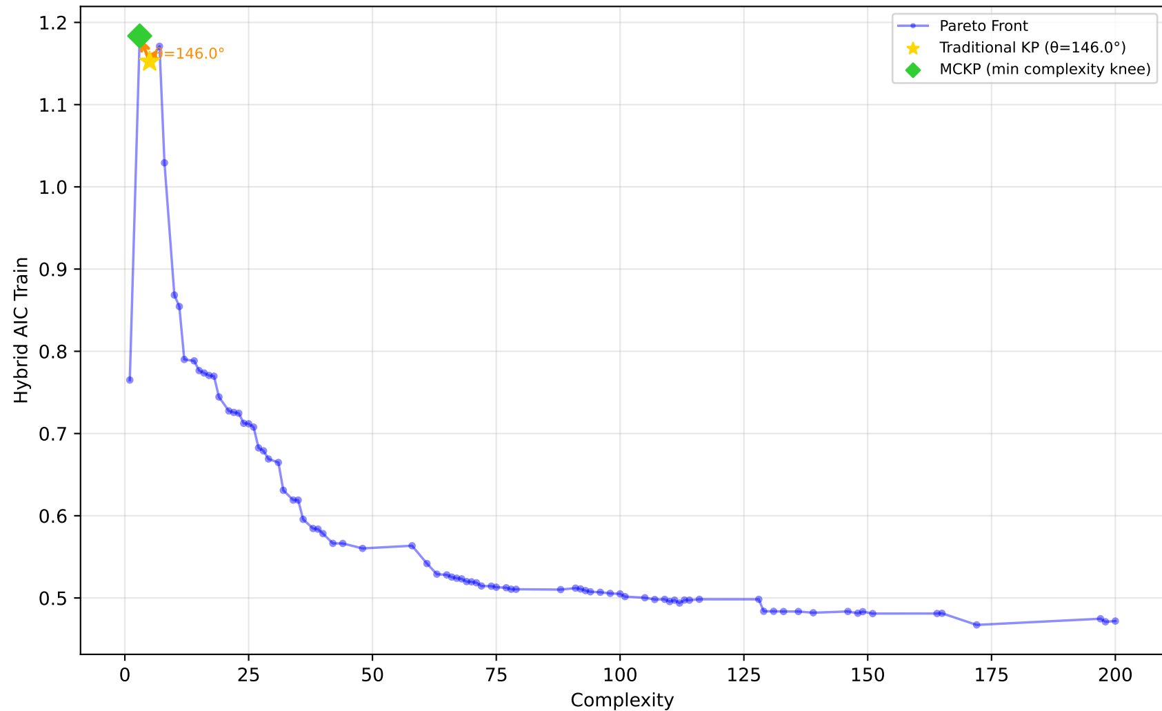
561_cpu - Run 5 - SVP - Hybrid AIC Train \lambda_1=0.90 , \lambda_2=0.00 , \lambda_3=0.30 | Difficulty: 1.00 | Method: hmr
