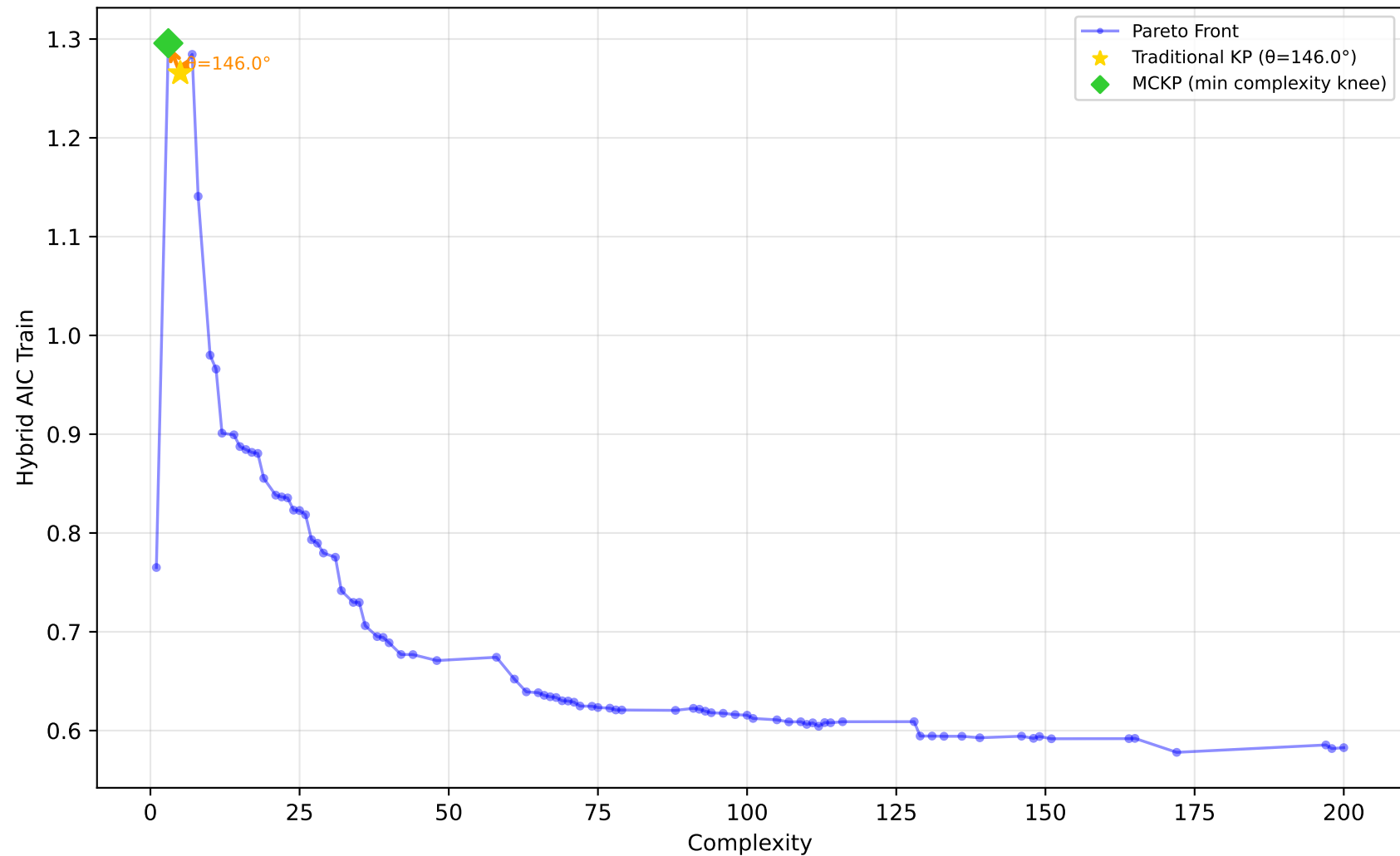
561_cpu - Run 5 - SVP - Hybrid AIC Train \lambda_1=1.00, \lambda_2=0.00, \lambda_3=0.40 | Difficulty: 1.00 | Method: hmr
