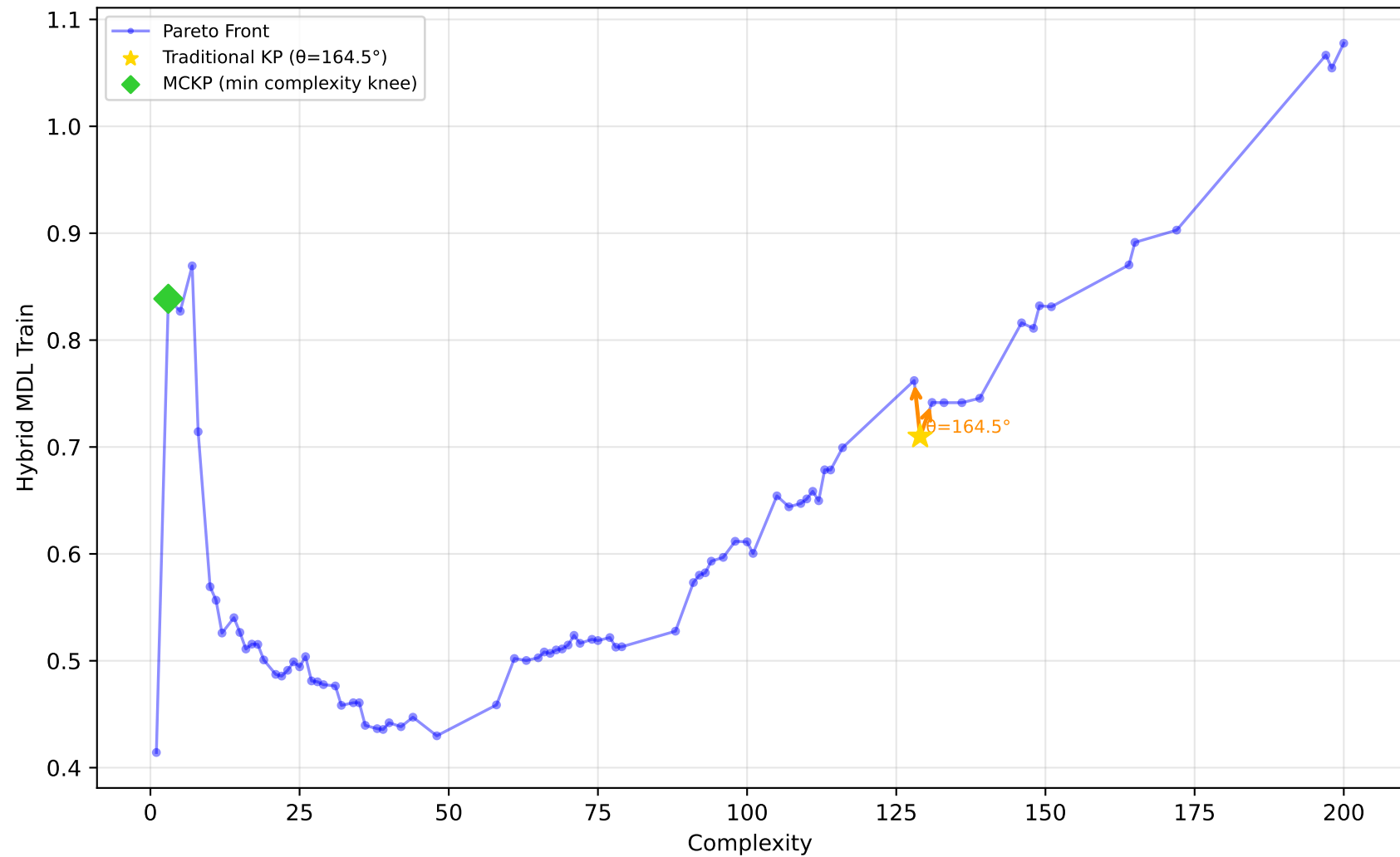
561_cpu - Run 5 - SVP - Hybrid MDL Train \lambda_1=0.90, \lambda_2=0.00, \lambda_3=0.30 | Difficulty: 1.00 | Method: hmr
