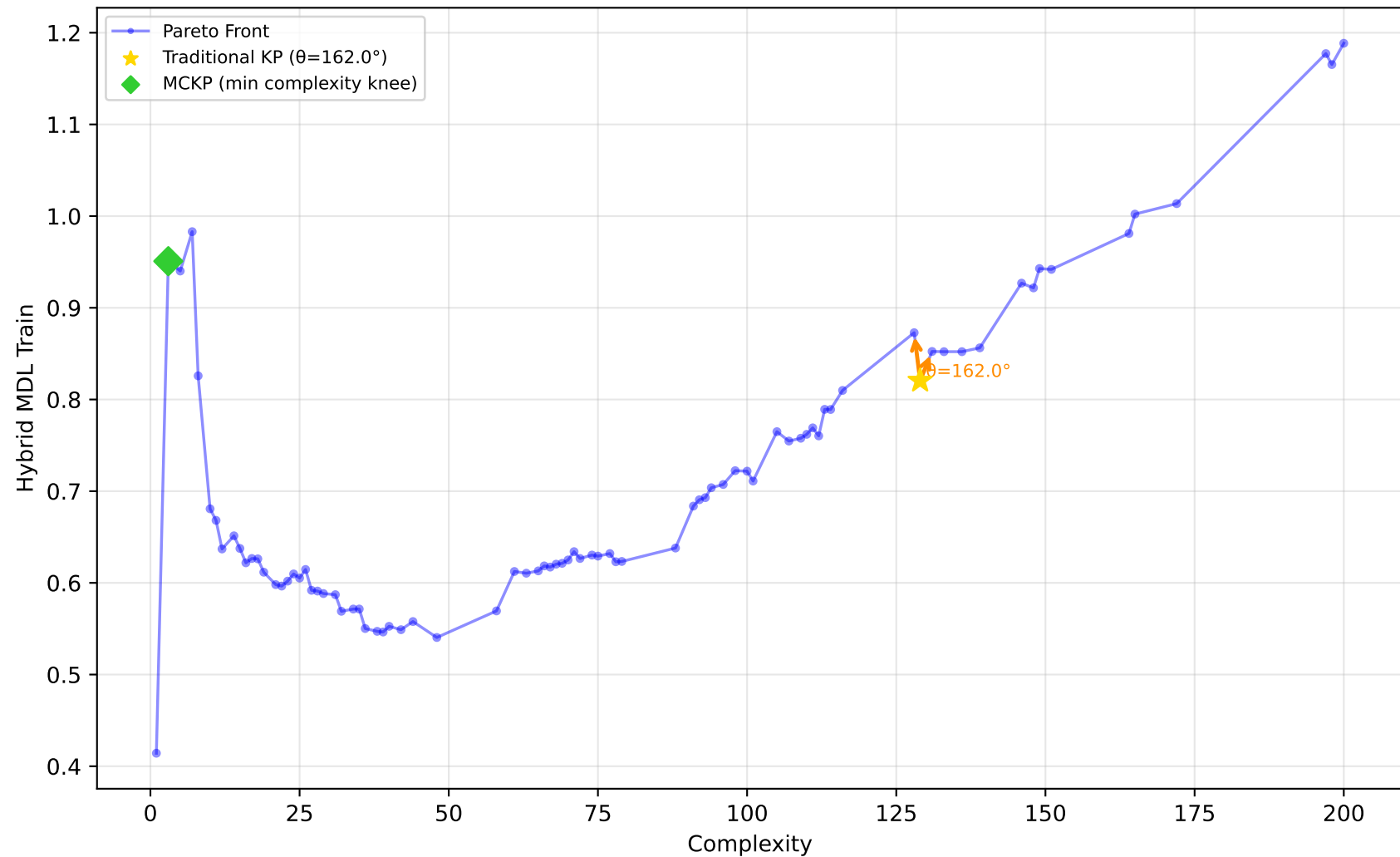
561_cpu - Run 5 - SVP - Hybrid MDL Train \lambda_1=1.00, \lambda_2=0.00, \lambda_3=0.40 | Difficulty: 1.00 | Method: hmr
