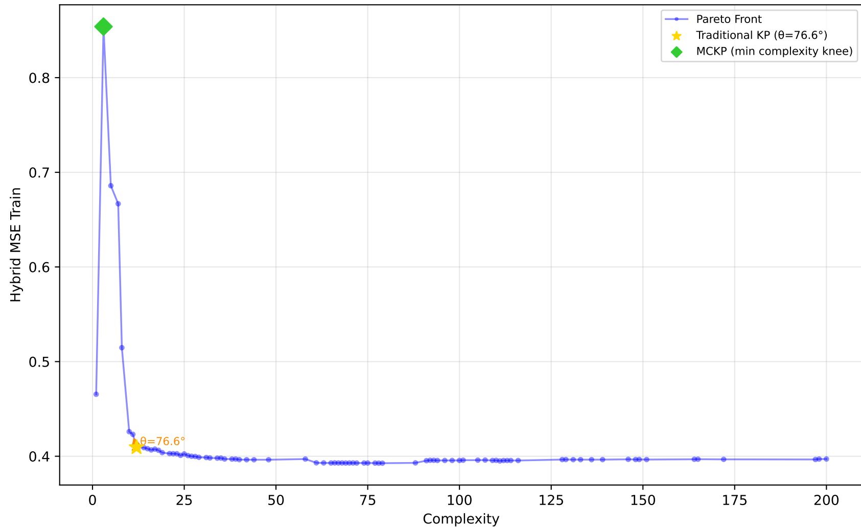
561_cpu - Run 5 - SVP - Hybrid MSE Train \lambda_1=0.90, \lambda_2=0.00, \lambda_3=0.30 | Difficulty: 1.00 | Method: hmr
