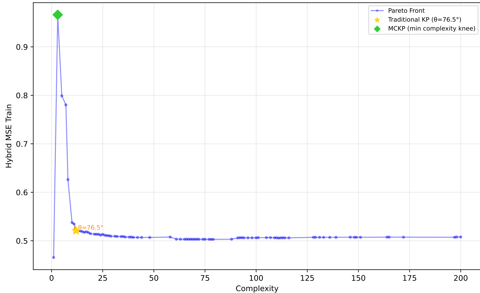
561_cpu - Run 5 - SVP - Hybrid MSE Train \lambda_1=1.00, \lambda_2=0.00, \lambda_3=0.40 | Difficulty: 1.00 | Method: hmr
