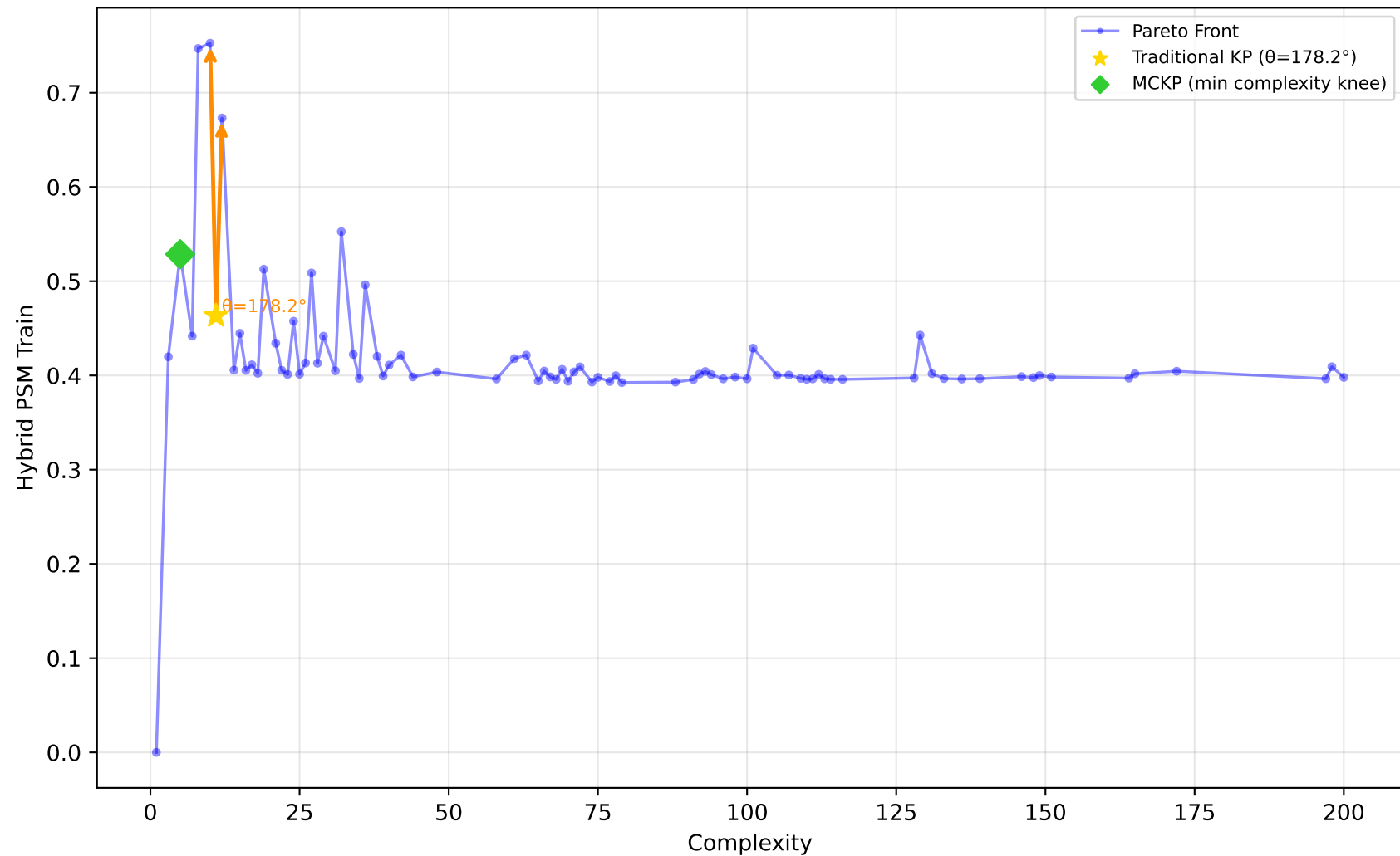
561_cpu - Run 5 - SVP - Hybrid PSM Train \lambda_1=0.90, \lambda_2=0.00, \lambda_3=0.30 | Difficulty: 1.00 | Method: hmr
