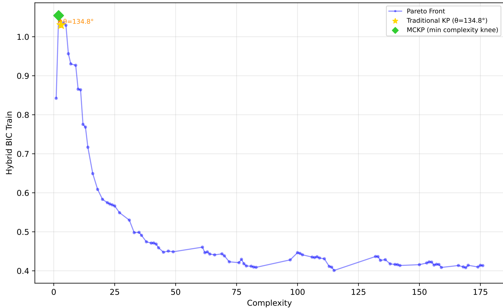
561_cpu - Run 6 - MVP - Hybrid BIC Train \lambda_1=0.50, \lambda_2=0.20, \lambda_3=0.00 | Difficulty: 1.00 | Method: hmr
