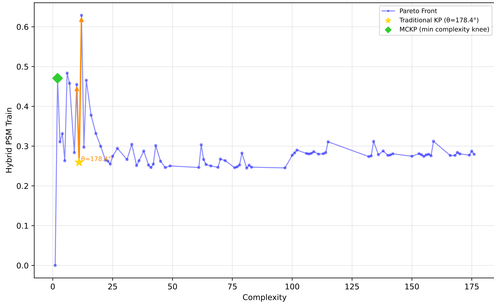
561_cpu - Run 6 - MVP - Hybrid PSM Train \lambda_1=0.50, \lambda_2=0.20, \lambda_3=0.00 | Difficulty: 1.00 | Method: hmr
