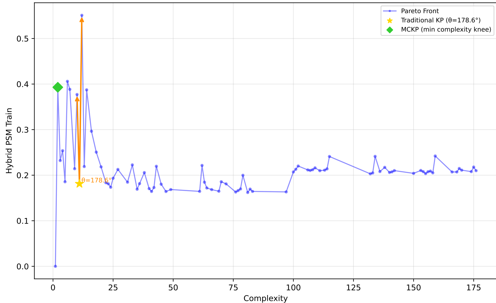
561_cpu - Run 6 - MVP - Hybrid PSM Train \lambda_1=0.70, \lambda_2=0.00, \lambda_3=0.10 | Difficulty: 1.00 | Method: hmr
