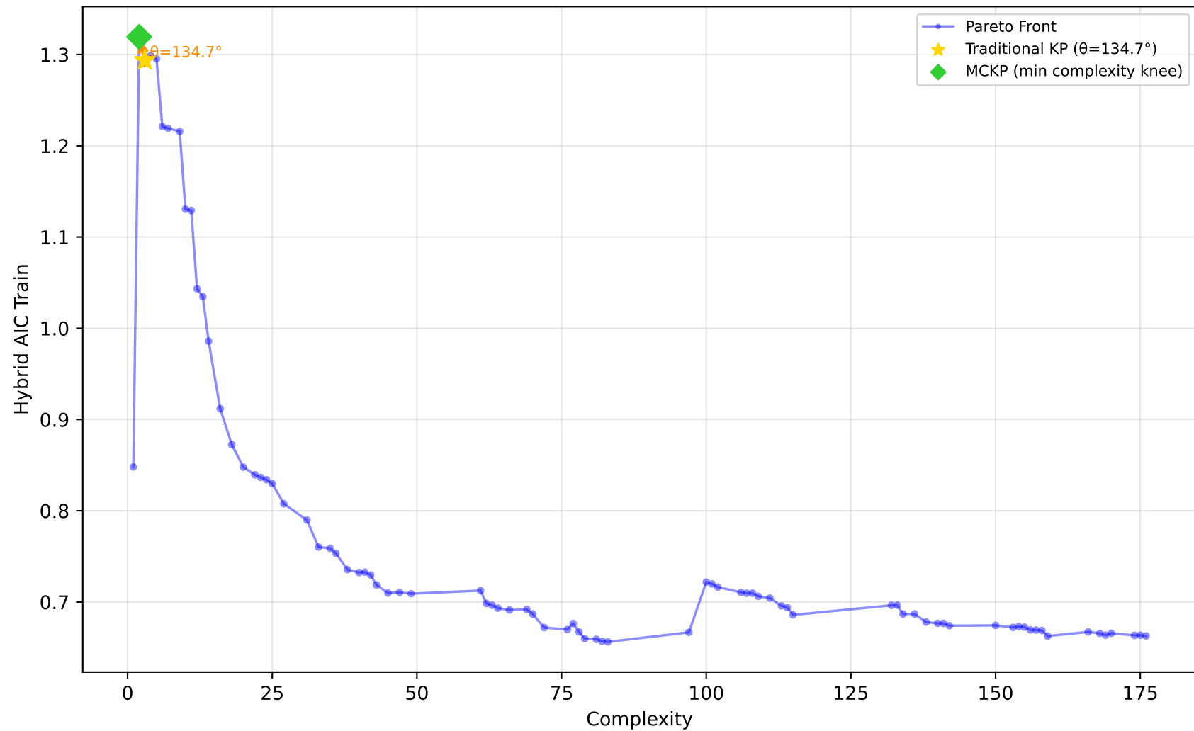
561_cpu - Run 6 - SVP - Hybrid AIC Train \lambda_1=1.00, \lambda_2=0.00, \lambda_3=0.40 | Difficulty: 1.00 | Method: hmr
