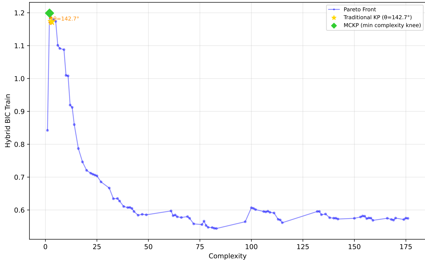
561_cpu - Run 6 - SVP - Hybrid BIC Train \lambda_1=0.90, \lambda_2=0.00, \lambda_3=0.30 | Difficulty: 1.00 | Method: hmr
