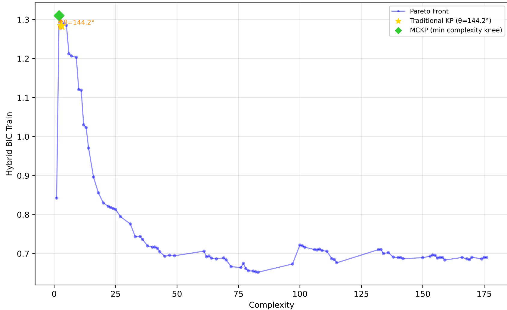
561_cpu - Run 6 - SVP - Hybrid BIC Train \lambda_1=1.00, \lambda_2=0.00, \lambda_3=0.40 | Difficulty: 1.00 | Method: hmr
