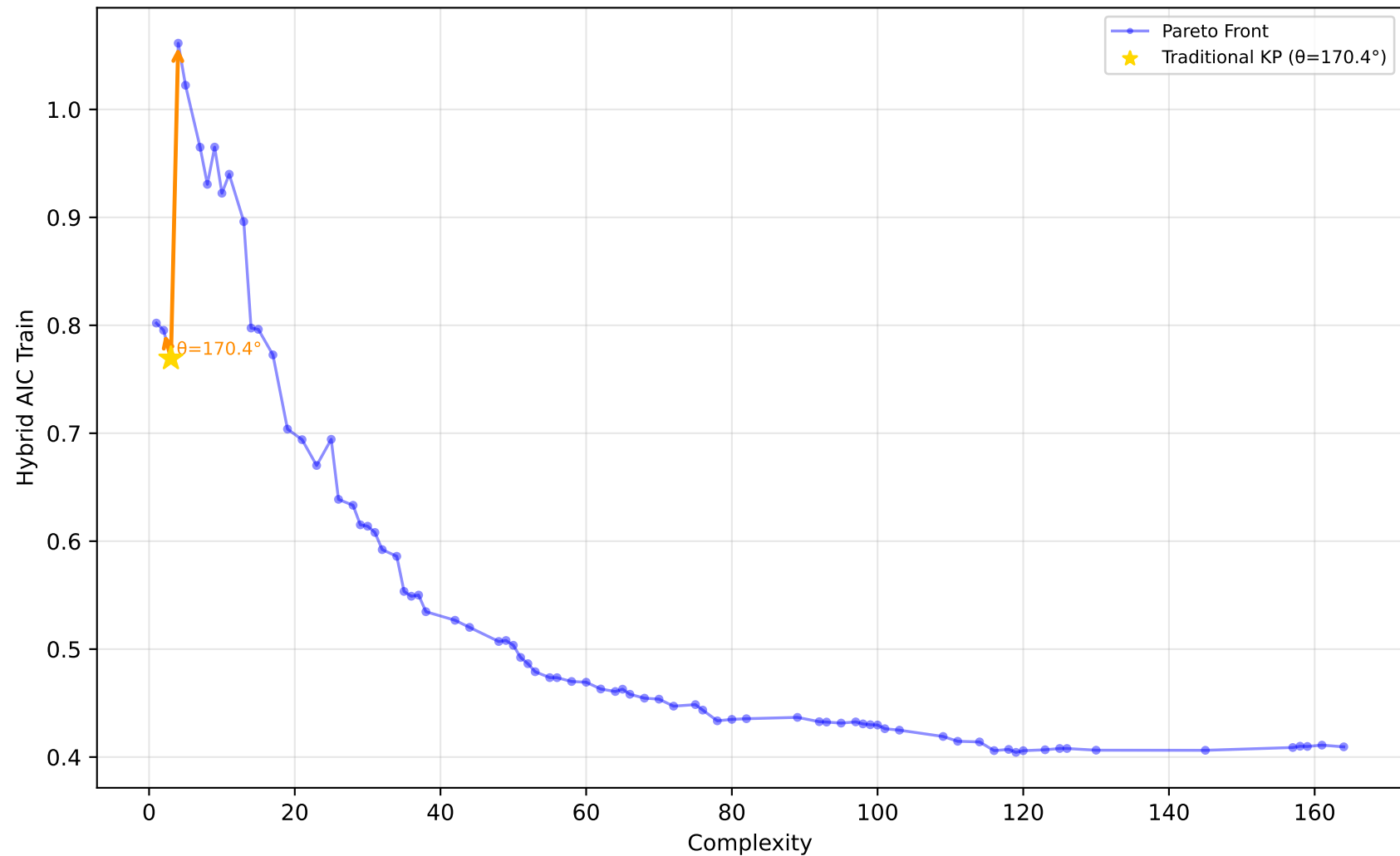
561_cpu - Run 7 - MVP - Hybrid AIC Train \lambda_1=0.50, \lambda_2=0.20, \lambda_3=0.00 | Difficulty: 1.00 | Method: hmr
