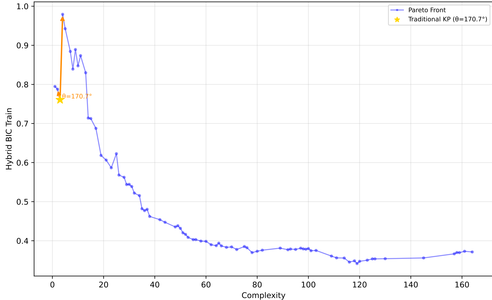
561_cpu - Run 7 - MVP - Hybrid BIC Train \lambda_1=0.70, \lambda_2=0.00, \lambda_3=0.10 | Difficulty: 1.00 | Method: hmr
