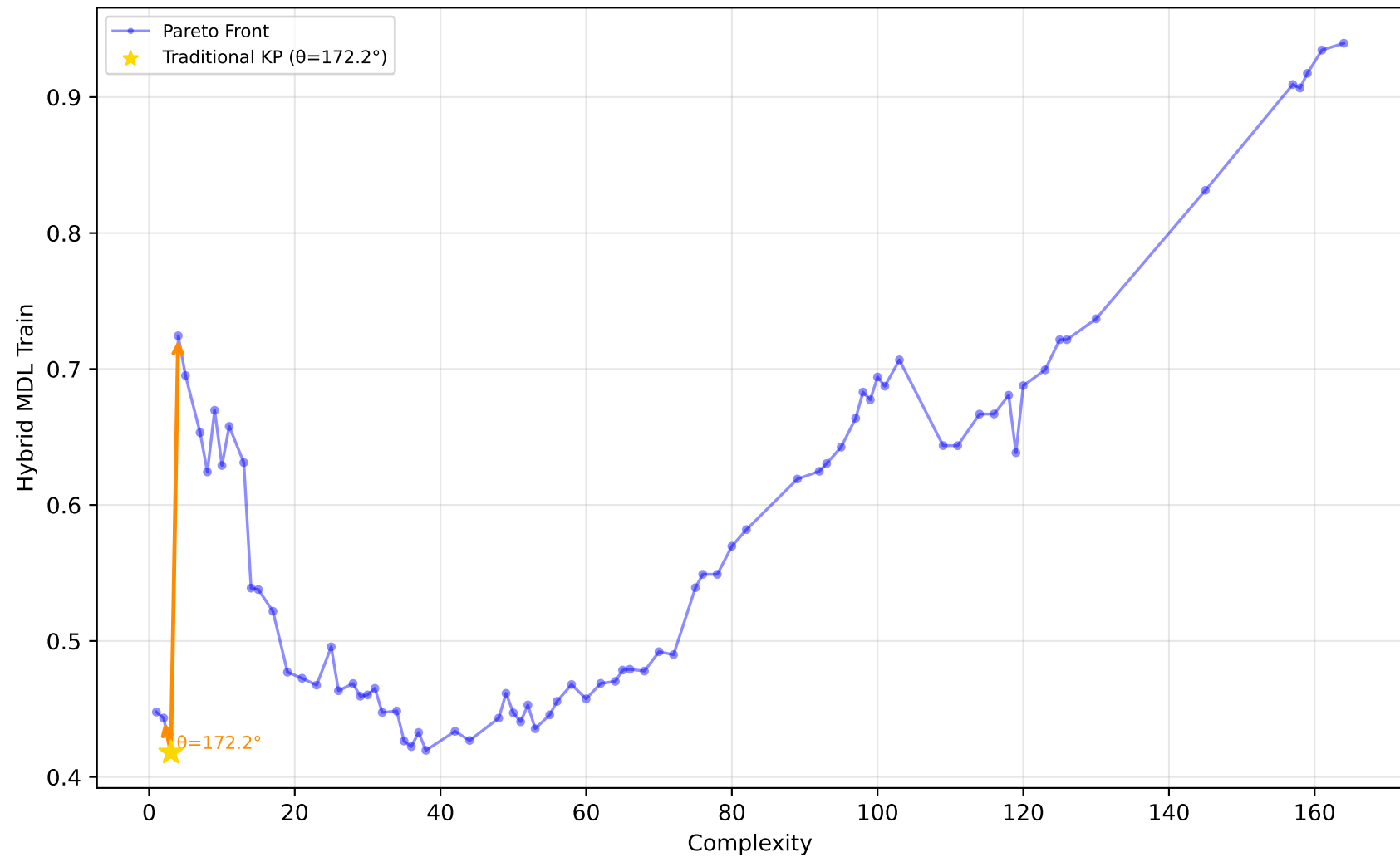
561_cpu - Run 7 - MVP - Hybrid MDL Train \lambda_1=0.50, \lambda_2=0.20, \lambda_3=0.00 | Difficulty: 1.00 | Method: hmr
