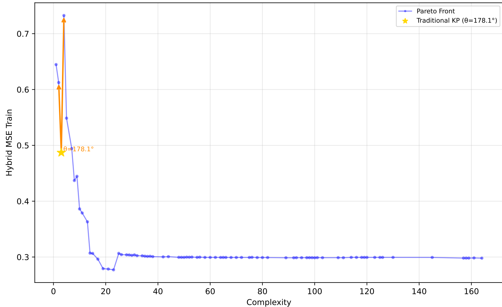
561_cpu - Run 7 - MVP - Hybrid MSE Train \lambda_1=0.50, \lambda_2=0.20, \lambda_3=0.00 | Difficulty: 1.00 | Method: hmr
