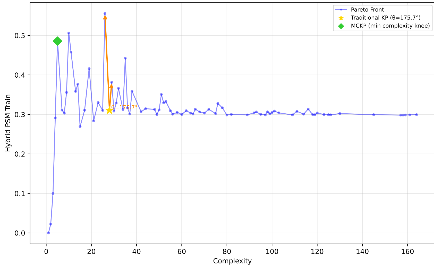
561_cpu - Run 7 - MVP - Hybrid PSM Train \lambda_1=0.50, \lambda_2=0.20, \lambda_3=0.00 | Difficulty: 1.00 | Method: hmr
