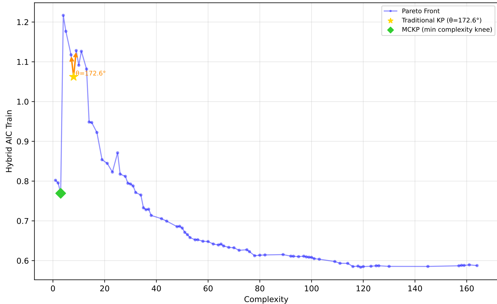
561_cpu - Run 7 - SVP - Hybrid AIC Train \lambda_1=0.90, \lambda_2=0.00, \lambda_3=0.30 | Difficulty: 1.00 | Method: hmr
