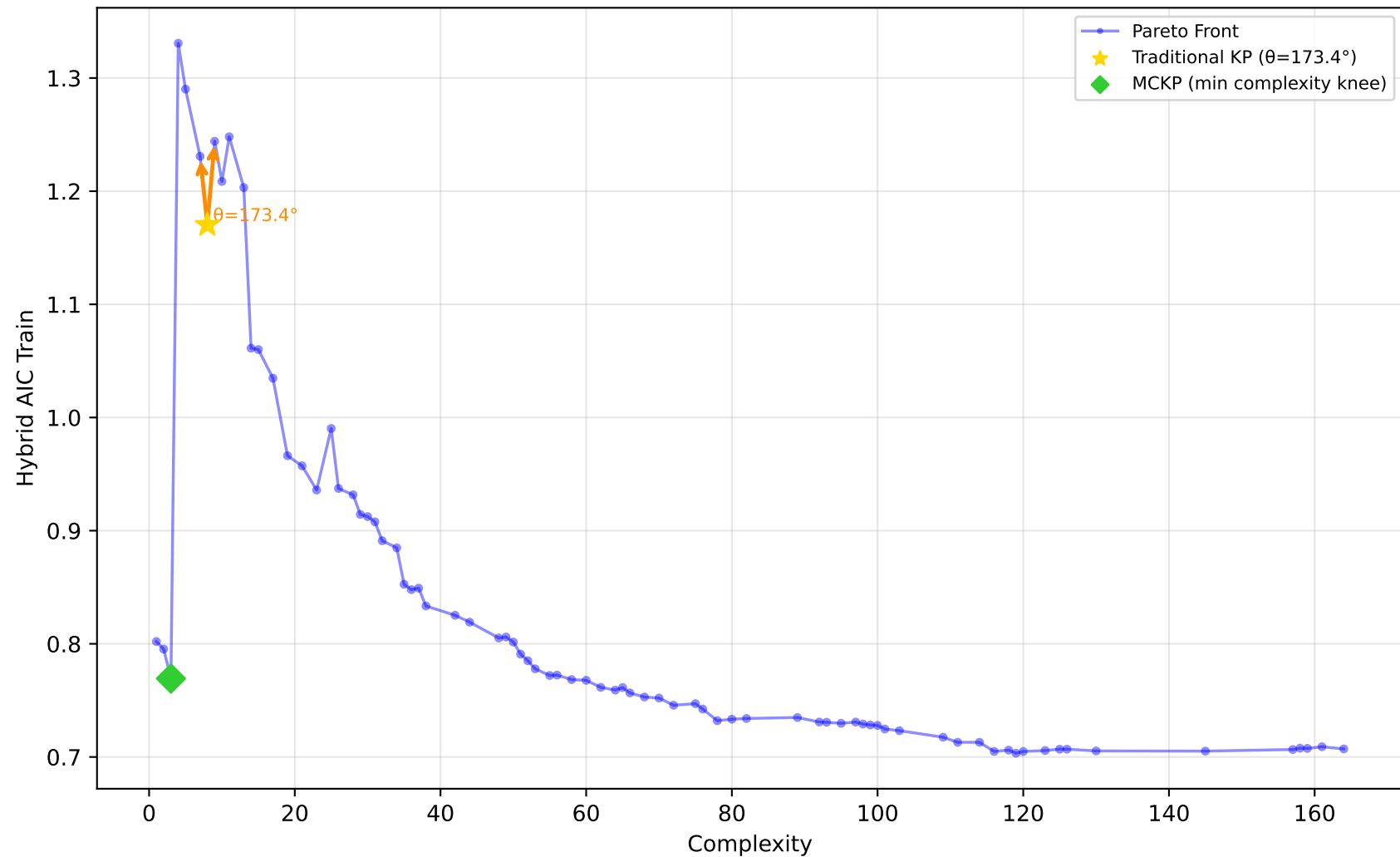
561_cpu - Run 7 - SVP - Hybrid AIC Train \lambda_1=1.00, \lambda_2=0.00, \lambda_3=0.40 | Difficulty: 1.00 | Method: hmr
