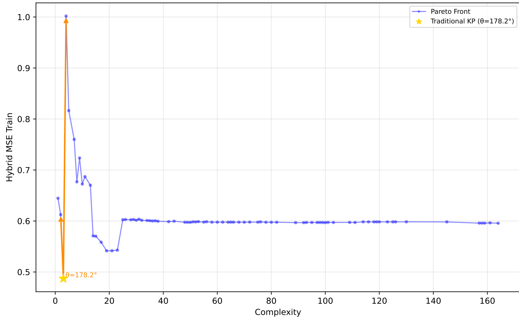
561_cpu - Run 7 - SVP - Hybrid MSE Train \lambda_1=1.00, \lambda_2=0.00, \lambda_3=0.40 | Difficulty: 1.00 | Method: hmr
