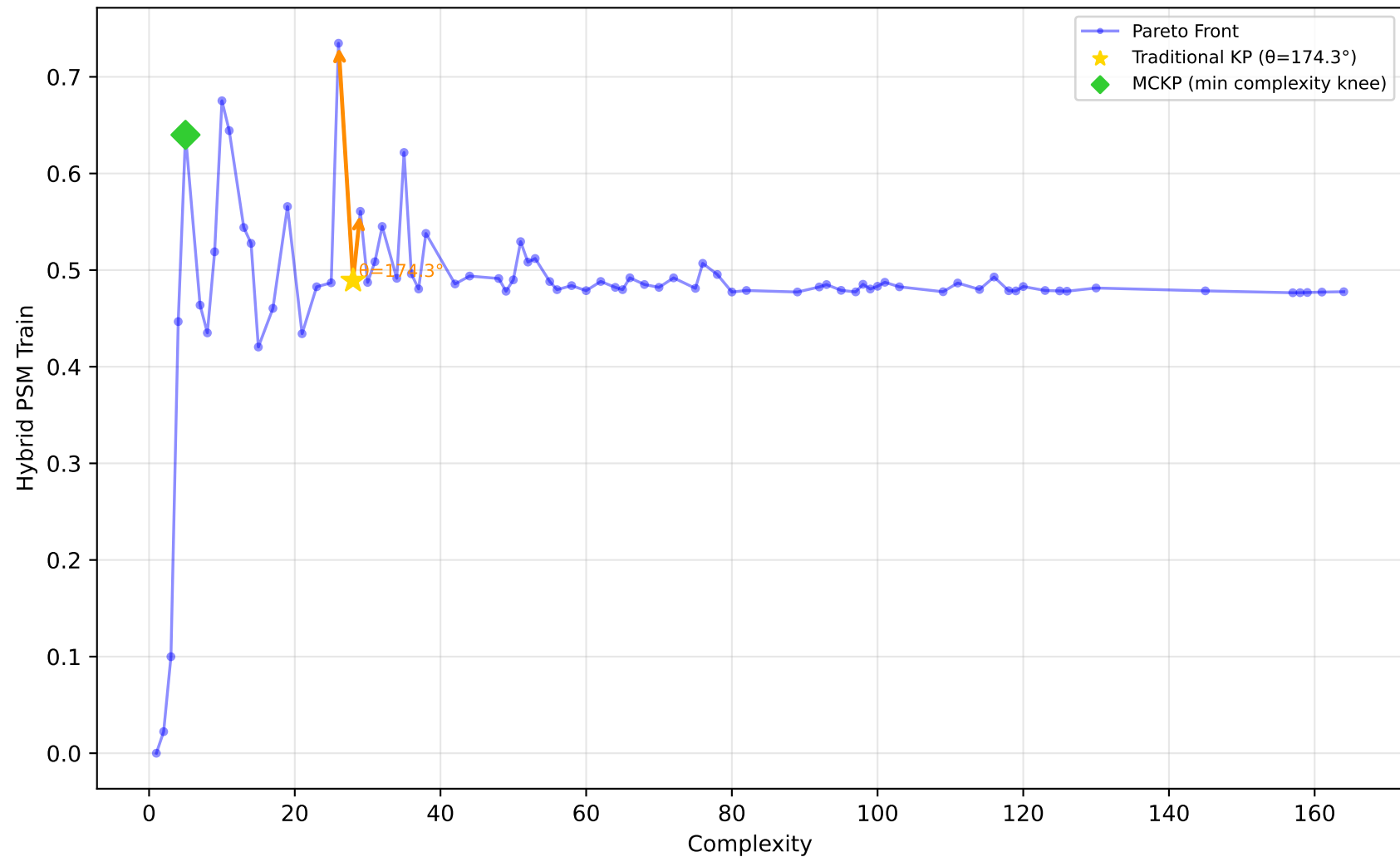
561_cpu - Run 7 - SVP - Hybrid PSM Train \lambda_1=0.90, \lambda_2=0.00, \lambda_3=0.30 | Difficulty: 1.00 | Method: hmr
