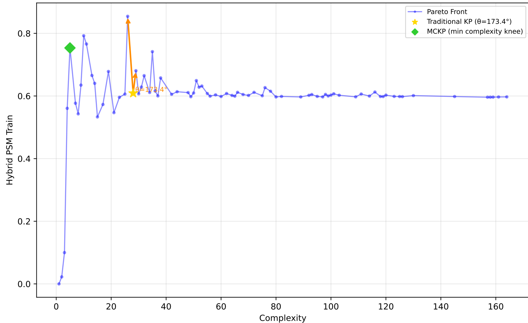
561_cpu - Run 7 - SVP - Hybrid PSM Train \lambda_1=1.00, \lambda_2=0.00, \lambda_3=0.40 | Difficulty: 1.00 | Method: hmr
