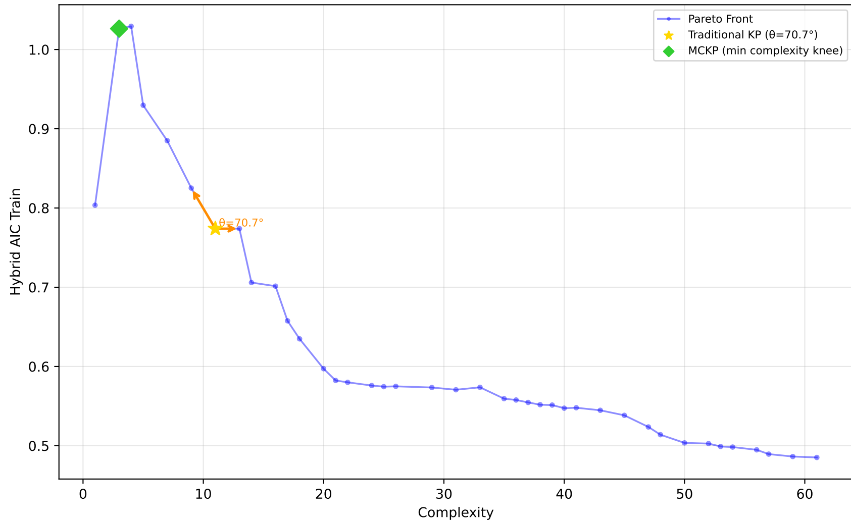
561_cpu - Run 8 - MVP - Hybrid AIC Train \lambda_1=0.50, \lambda_2=0.20, \lambda_3=0.00 | Difficulty: 1.00 | Method: hmr
