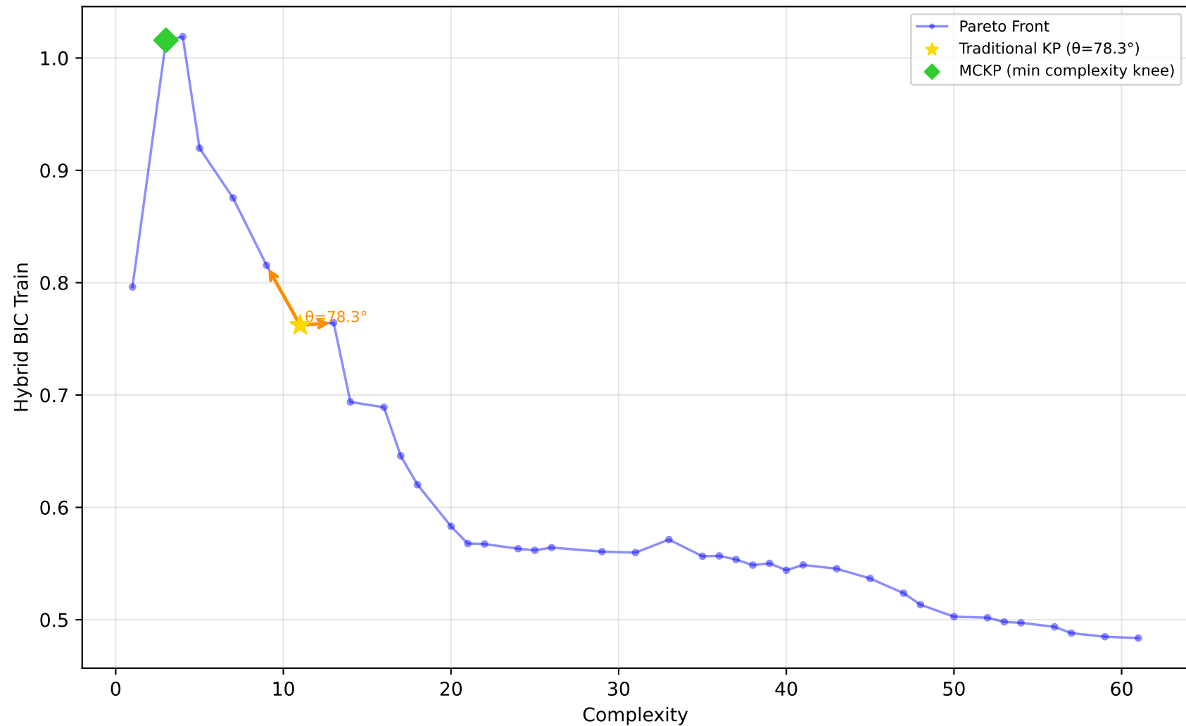
561_cpu - Run 8 - MVP - Hybrid BIC Train \lambda_1=0.50, \lambda_2=0.20, \lambda_3=0.00 | Difficulty: 1.00 | Method: hmr
