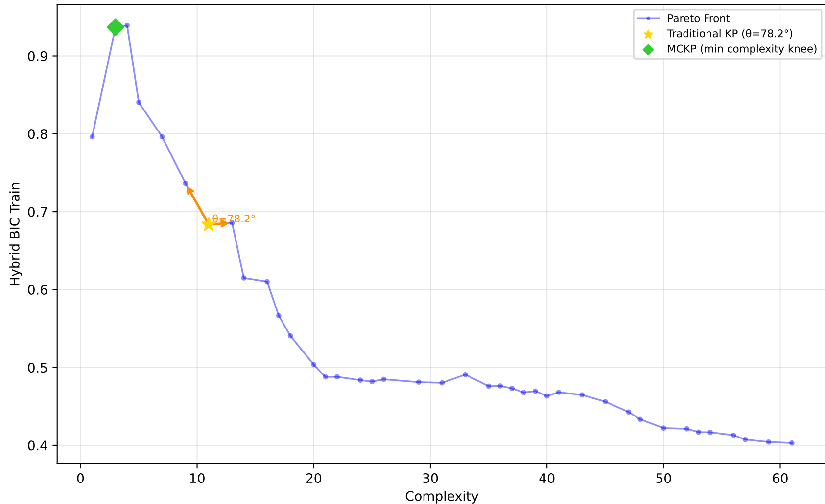
561_cpu - Run 8 - MVP - Hybrid BIC Train \lambda_1=0.70, \lambda_2=0.00, \lambda_3=0.10 | Difficulty: 1.00 | Method: hmr
