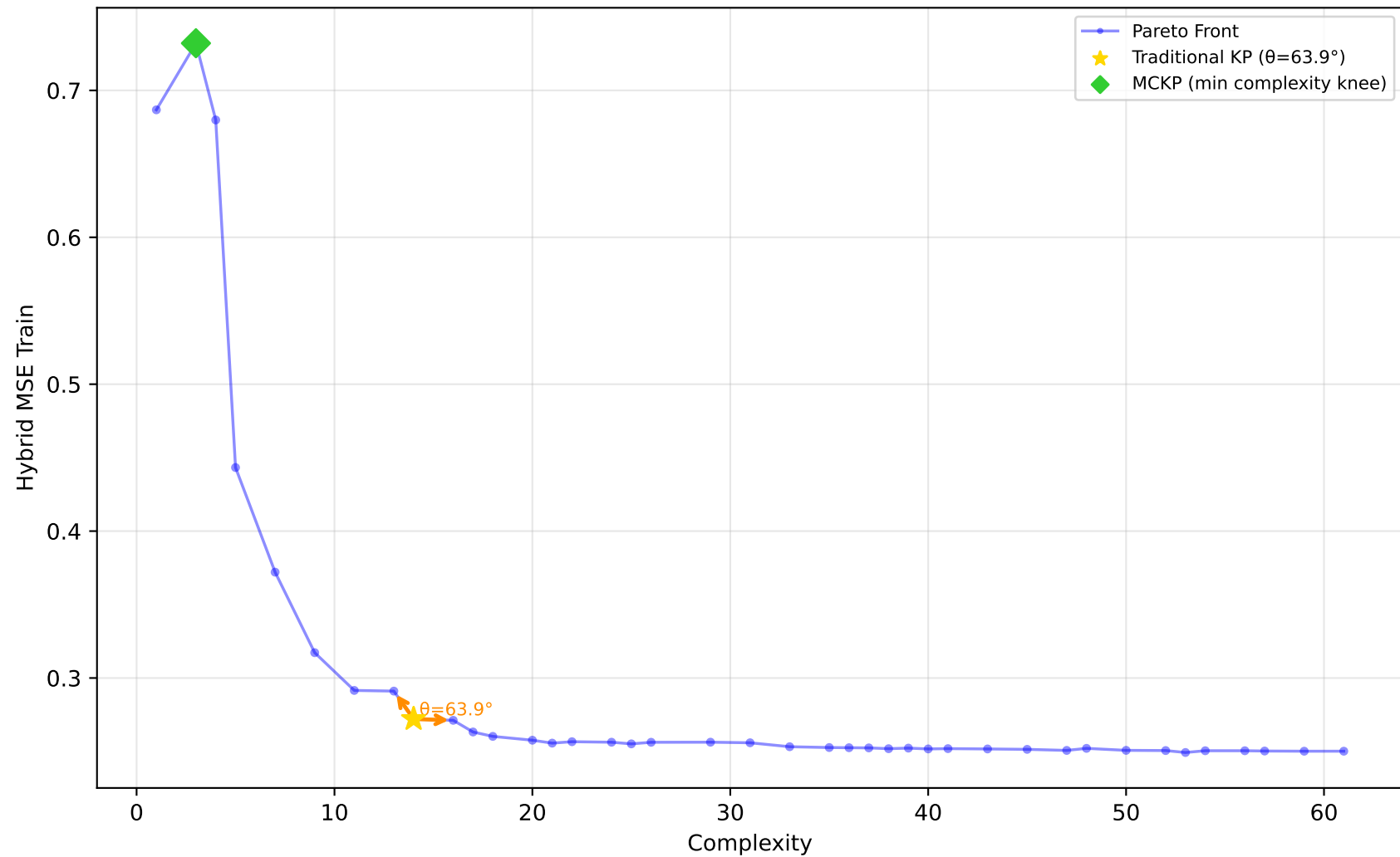
561_cpu - Run 8 - MVP - Hybrid MSE Train \lambda_1=0.50, \lambda_2=0.20, \lambda_3=0.00 | Difficulty: 1.00 | Method: hmr
