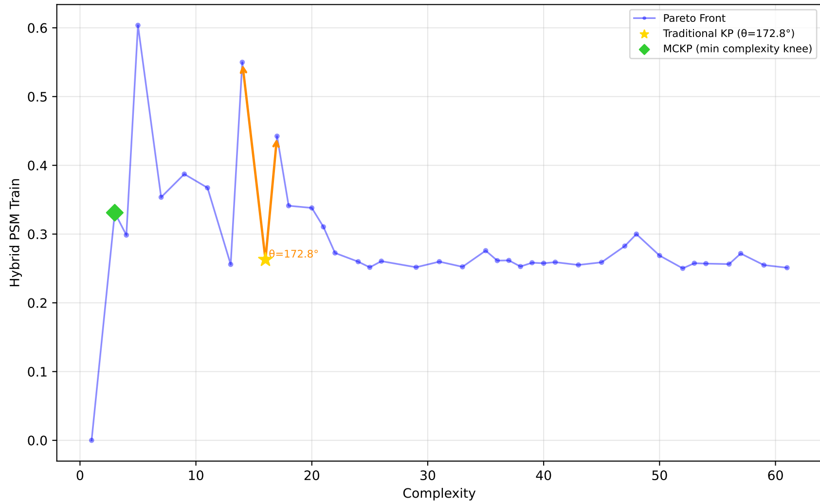
561_cpu - Run 8 - MVP - Hybrid PSM Train \lambda_1=0.50, \lambda_2=0.20, \lambda_3=0.00 | Difficulty: 1.00 | Method: hmr
