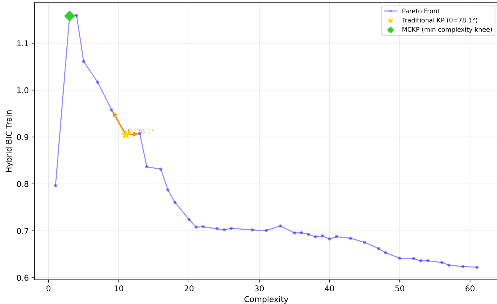
561_cpu - Run 8 - SVP - Hybrid BIC Train \lambda_1=0.90, \lambda_2=0.00, \lambda_3=0.30 | Difficulty: 1.00 | Method: hmr
