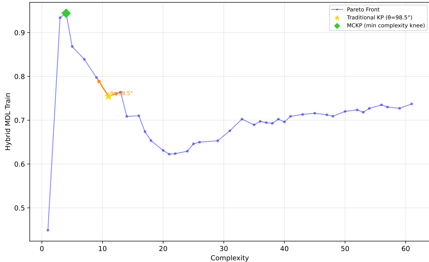
561_cpu - Run 8 - SVP - Hybrid MDL Train \lambda_1=1.00, \lambda_2=0.00, \lambda_3=0.40 | Difficulty: 1.00 | Method: hmr
