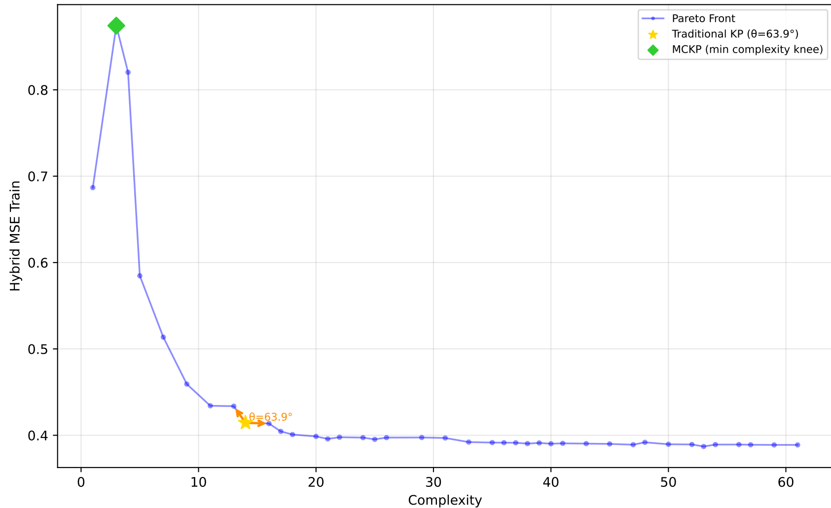
561_cpu - Run 8 - SVP - Hybrid MSE Train \lambda_1=0.90, \lambda_2=0.00, \lambda_3=0.30 | Difficulty: 1.00 | Method: hmr
