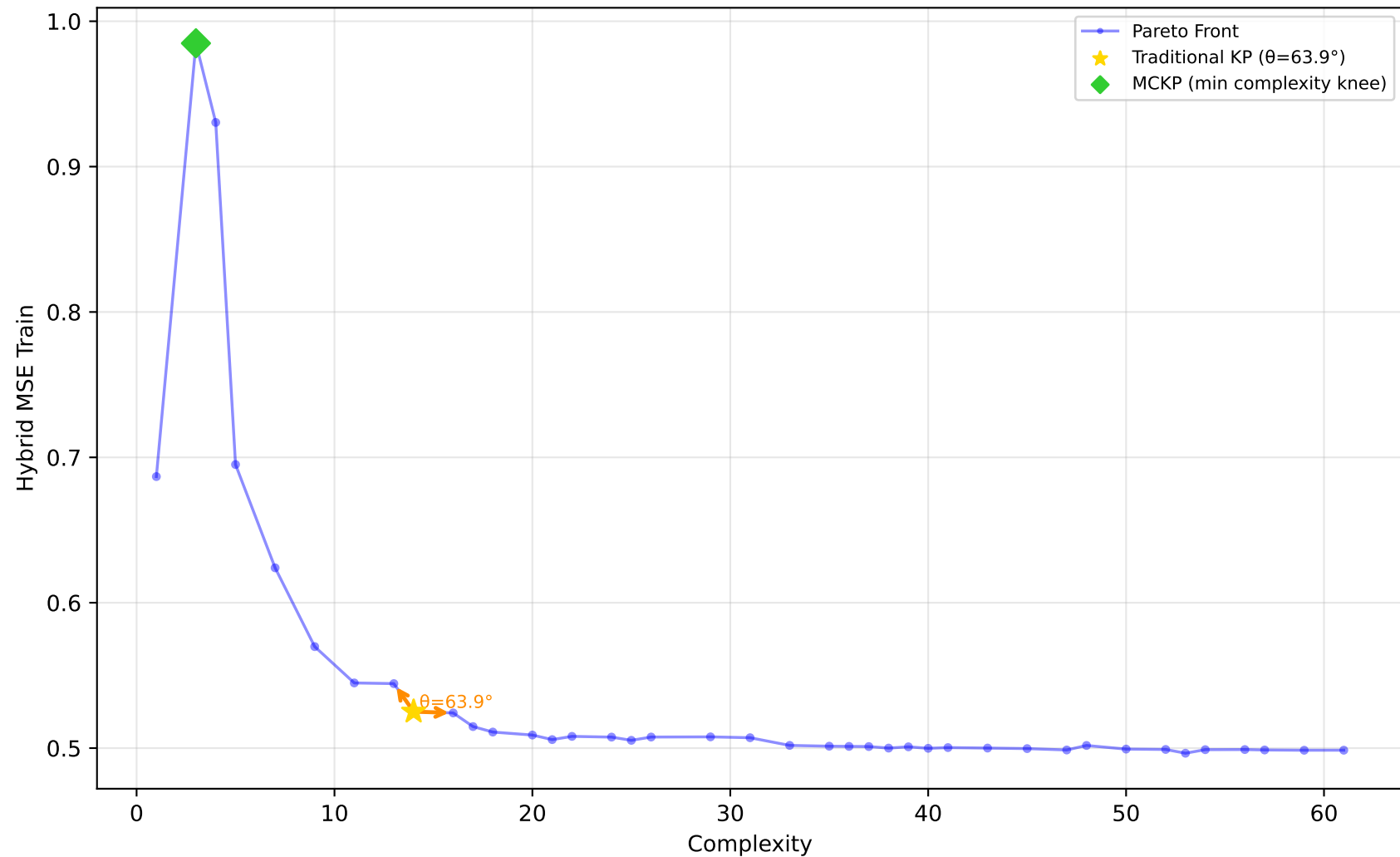
561_cpu - Run 8 - SVP - Hybrid MSE Train \lambda_1=1.00, \lambda_2=0.00, \lambda_3=0.40 | Difficulty: 1.00 | Method: hmr
