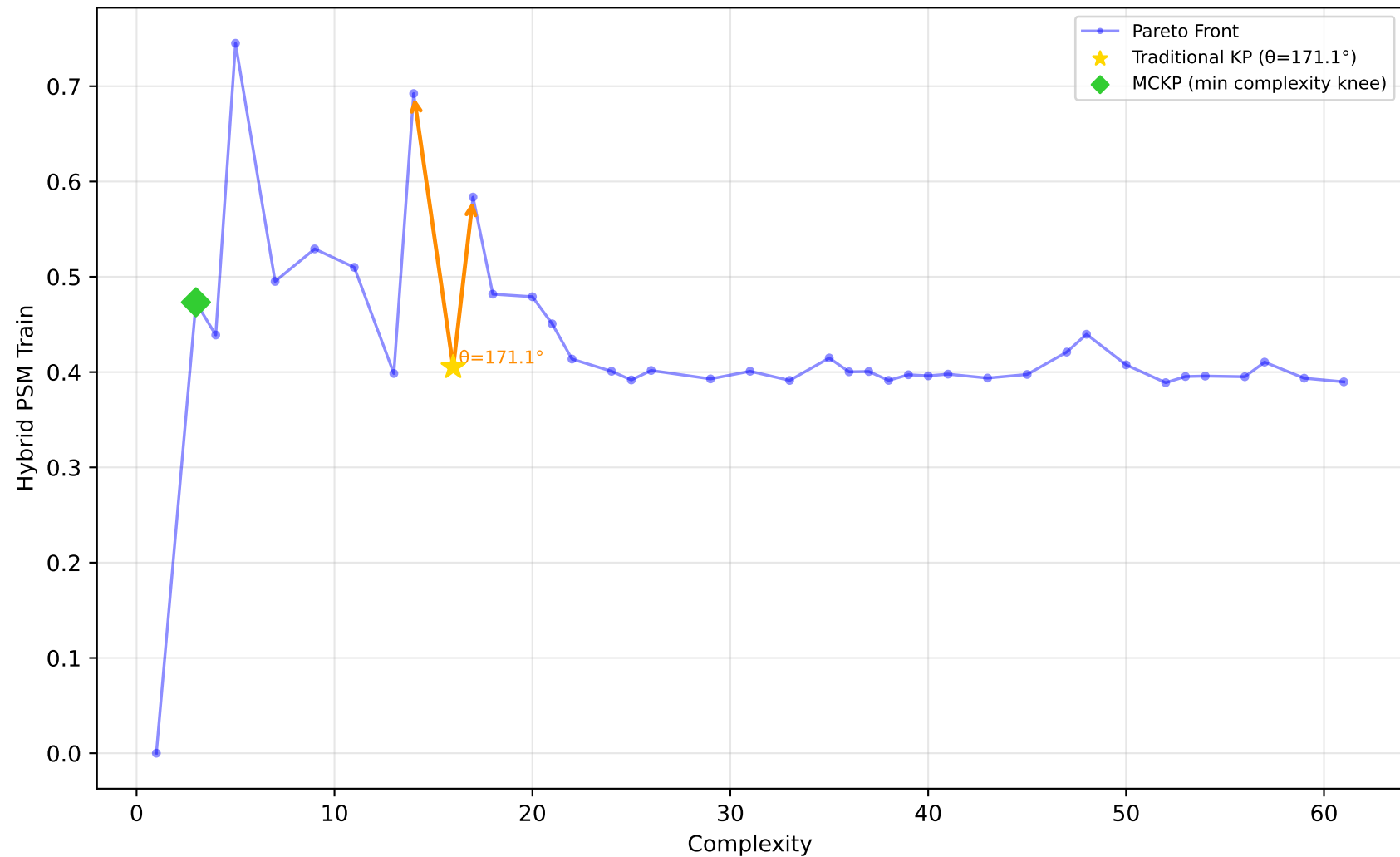
561_cpu - Run 8 - SVP - Hybrid PSM Train \lambda_1=0.90, \lambda_2=0.00, \lambda_3=0.30 | Difficulty: 1.00 | Method: hmr
