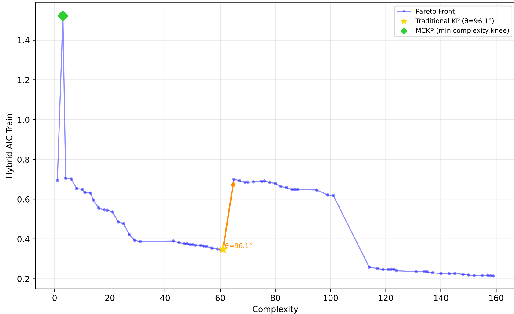
561_cpu - Run 9 - MVP - Hybrid AIC Train \lambda_1=0.70, \lambda_2=0.00, \lambda_3=0.10 | Difficulty: 0.55 | Method: mckp
