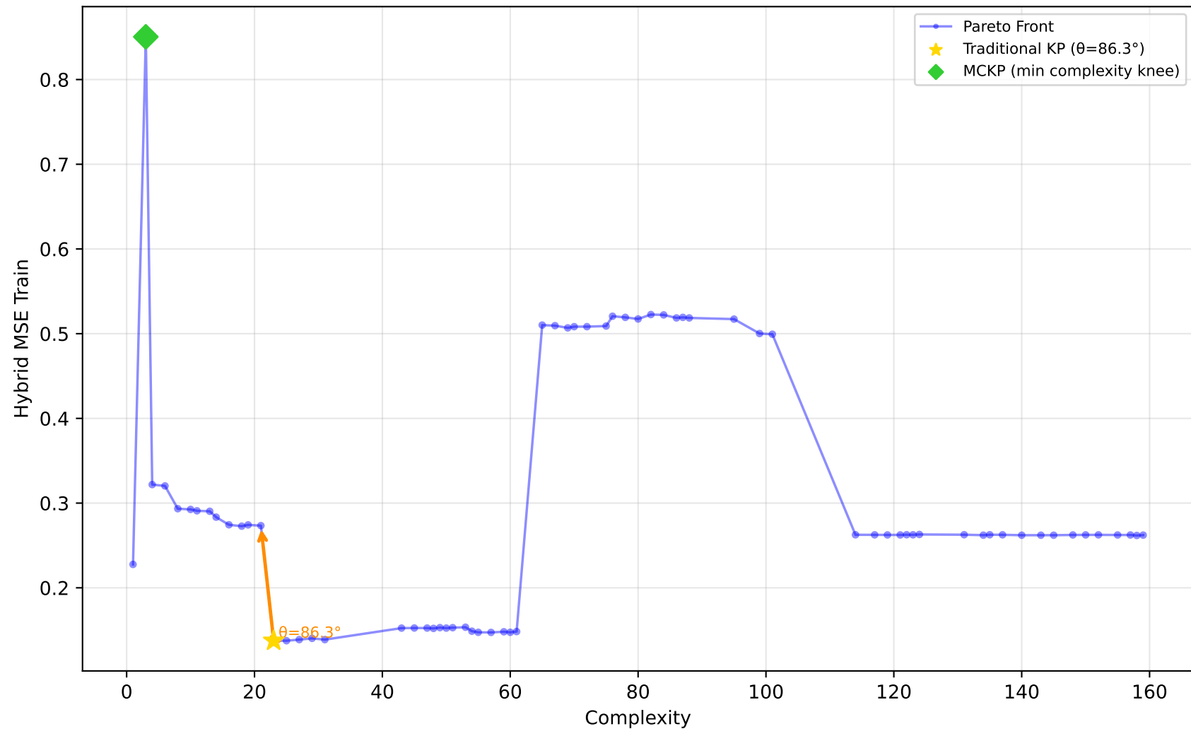
561_cpu - Run 9 - MVP - Hybrid MSE Train \lambda_1=0.50, \lambda_2=0.20, \lambda_3=0.00 | Difficulty: 0.55 | Method: mckp
